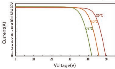
IV Curves of JT540SGh at different Temp
