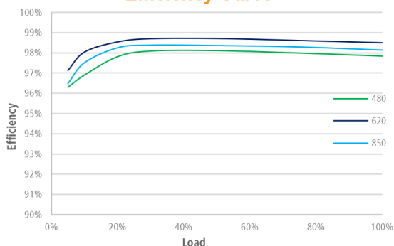
Efficiency Curve
